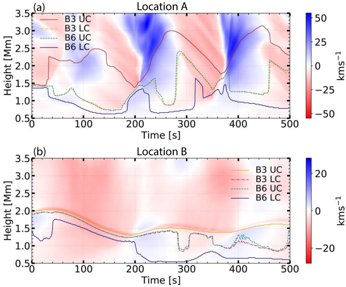
Fig. A.1. Time evolution of the vertical velocities of the columns at location A during the propagation of shock waves (a) and at location B in the network region (b). Upwards motion, away from the photosphere, is indicated by negative velocity (blue color). The representative heights of formation of the lower and upper components of the observables for bands 3 and 6 are marked by the solid and dashed lines, respectively (see Sect. 3 in the main text for details).
