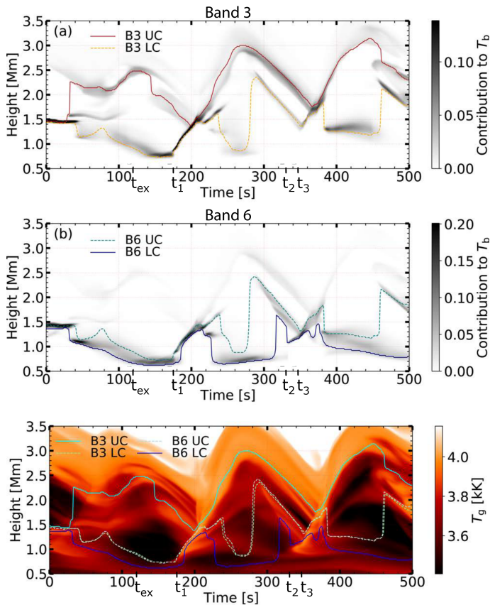
Fig. 3. Time evolution of contribution functions and plasma temperature for a column in the quiet Sun, at location A (Fig. 1), with the shock wave event studied in detail in Eklund et al. (2021a). Contribution function of band 3 (a) and band 6 (b) with the heights of 0.25 and 0.80 times the contribution function integrated from the top marked by the dashed and solid lines, respectively. (c) Plasma temperature with each of the representative heights of the two components of bands 3 and 6 marked for reference. The ticks t_{\text{ex}} and t_1 - t_3 mark the times for in-depth discussion in connection to Fig. 4 and Fig. 7.
