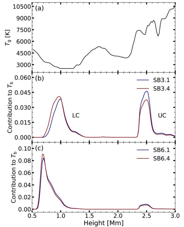
Fig. 4. Plasma temperature and contribution functions plotted against height in the atmosphere for one time step, t_{\text{ex}} = 120 s, of the shock wave (cf. Fig. 3) at location A (Fig. 1). (a) Plasma temperature as function of height. (b) Contribution functions of SB3.1 and SB3.4, each showing a lower and an upper component, marked LC and UC, respectively. (c) Contribution functions of SB6.1 and SB6.4.
