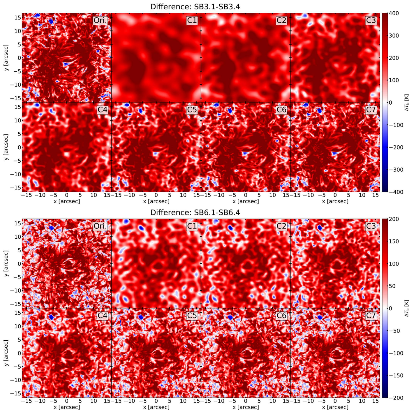
Fig. 9. The sub-band brightness temperature difference at band 3, \Delta T_b|_{B3} , (top panels) and at band 6, \Delta T_b|_{B6} , (bottom panels) at original resolution of the numerical model and at the resolutions corresponding to array configurations C1 to C7 for respective receiver sub-band (Table B.1). It should be noted that the T_b maps are individually degraded to respective resolution before the differences are calculated.
