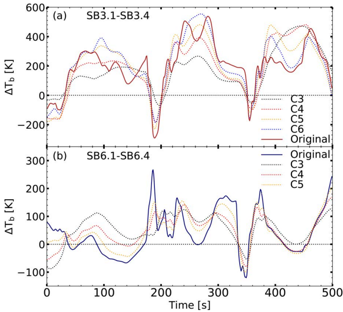
Fig. 10. Time evolution of the sub-band T_b differences of the time-series at location A at the different angular resolutions. (a) The T_b difference between sub-bands 3.1 and 3.4 at original resolution (solid red line) and at degraded resolutions corresponding to array configurations C3, C4, C5 and C6 (colored dotted lines). (b) T_b difference between sub-bands 6.1 and 6.4 at original resolution (solid blue line) and at degraded resolutions corresponding to array configurations C3, C4 and C5 (colored dotted lines). The horizontal black dotted lines show the level of \Delta T_b = 0 .
