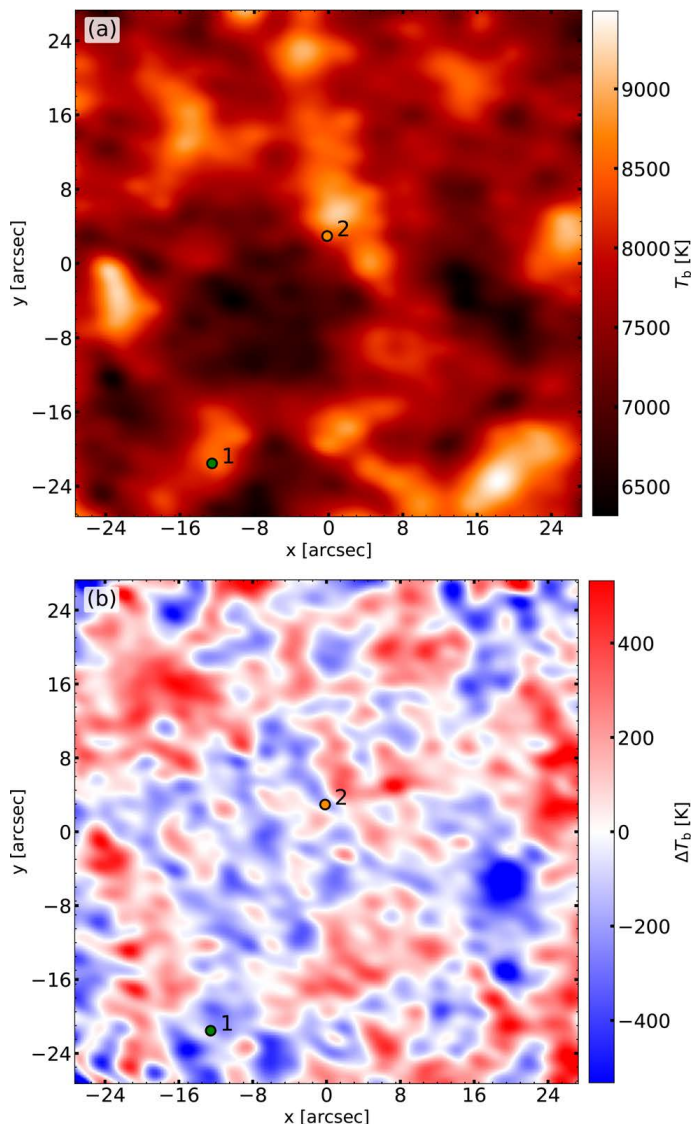
Fig. 11. Brightness temperature and sub-band brightness temperature difference of the FOV of the observational band 3 data at t = 290 s. (a) Brightness temperature of SB3.1, as constructed by adding the total power data to the interferometric data. (b) Difference of brightness temperature between the sub-bands, \Delta T_b|_{B3} = T_b|_{SB3.1} - T_b|_{SB3.4} , derived from only the interferometric data at each sub-band. The span of \Delta T_b|_{B3} is between -1150 K and 670 K, but the color scale was limited to -500 K to 500 K to reveal the small-scale structures. The locations of the two selected brightening events are marked by the green and orange markers, respectively.
