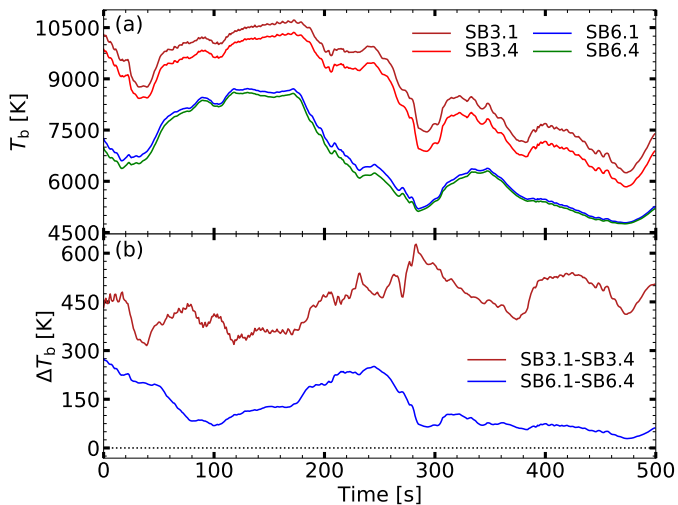
Fig. 8. Evolution of brightness temperatures and sub-band differences at location B in the network region between t = 0 –500 s. (a) The brightness temperatures of SB3.1, SB3.4, SB6.1 and SB6.4. (b) Sub-band differences \Delta T_{b|B3} ( T_{b|SB3.1} - T_{b|SB3.4} ) and \Delta T_{b|B6} ( T_{b|SB6.1} - T_{b|SB6.4} ).
