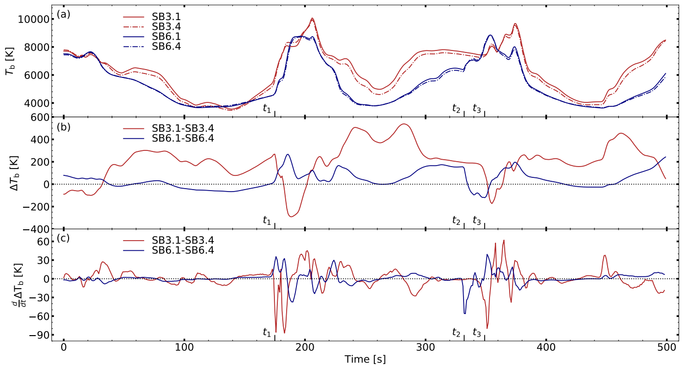
Fig. 7. Evolution of brightness temperatures and sub-band differences at the location of the propagating shock wave (location A) between t = 0 –500 s. (a) The brightness temperatures of SB3.1, SB3.4, SB6.1 and SB6.4. (b) Brightness temperature differences between the sub-bands \Delta T_{b|B3} ( T_{b|SB3.1} - T_{b|SB3.4} ) and \Delta T_{b|B6} ( T_{b|SB6.1} - T_{b|SB6.4} ). (c) Time-derivative of the sub-band differences \Delta T_{b|B3} and \Delta T_{b|B6} . In each panel, the time where the different bands starts to sample the shock waves are marked with the tick marks t_1 (bands 3 and 6), t_2 (band 6) and t_3 (band 3).
