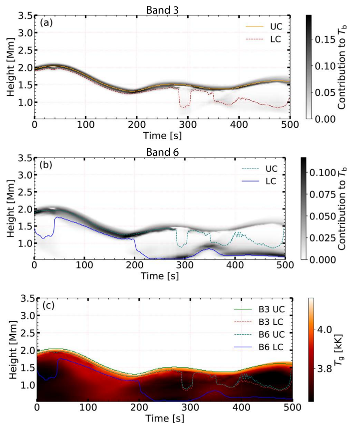
Fig. 5. Time evolution of contribution functions and plasma temperature for a column in the network patches at (x,y)=(3.8,4.2) arcsec, marked as location B at the FOV maps (Fig. 1). Top panel: Contribution function of band 3 with the heights of 0.25 and 0.8 times the contribution function integrated from the top marked by the dashed and solid lines, respectively. Middle panel: Same as top panel for band 6. Bottom panel: Plasma temperature with representative heights of formation of bands 3 and 6 marked with dashed and solid lines, respectively. The formation height at \tau = 1.0 of both sub-bands are indicated in respective row for ease of comparison.
