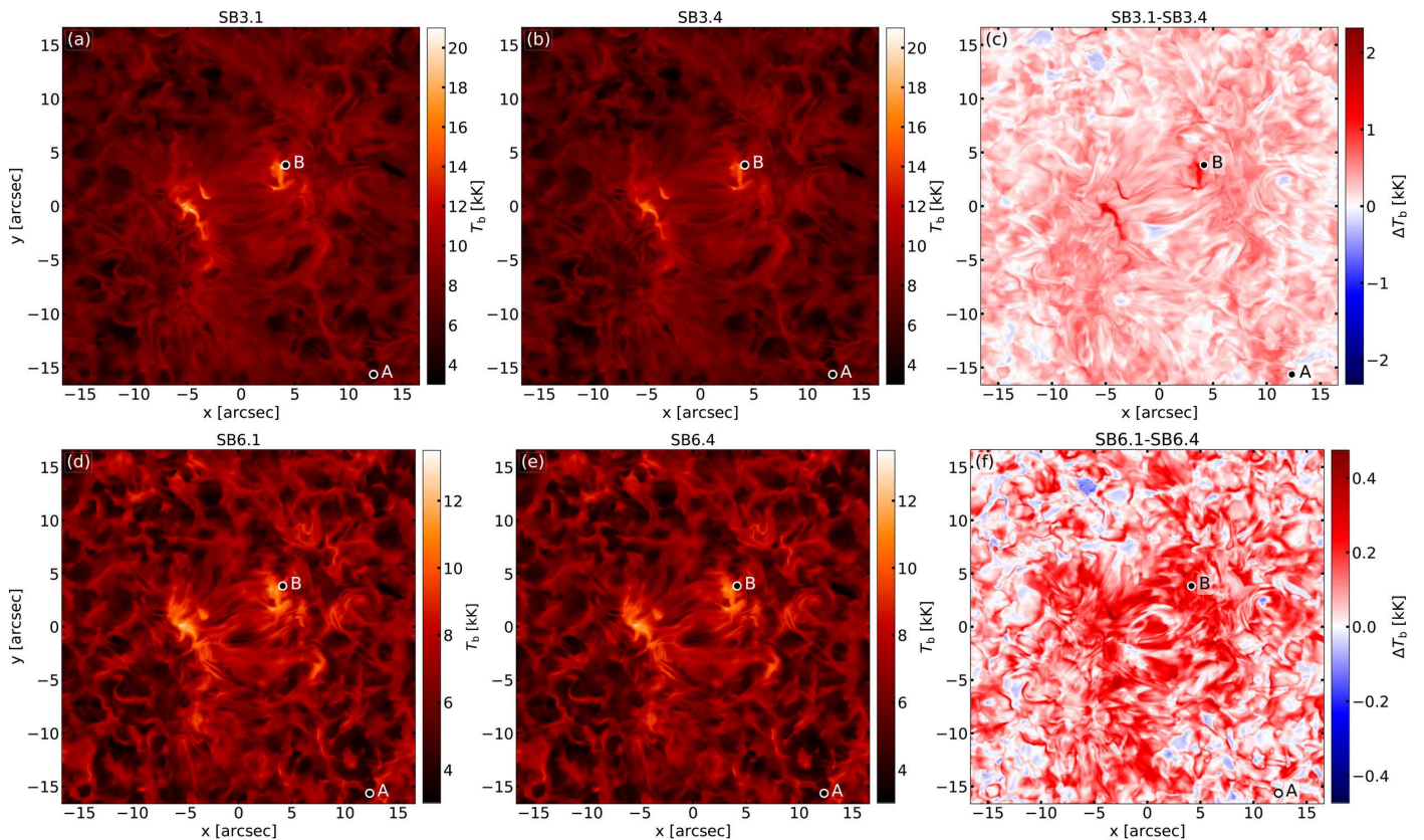
Fig. 6. Brightness temperatures of sub-bands of bands 3 and 6. (a) T_{b|SB3.1} , (b) T_{b|SB3.4} , (c) \Delta T_{b|B3} ( T_{b|SB3.1} - T_{b|SB3.4} ), (d) T_{b|SB6.1} , (e) T_{b|SB6.4} , (f) \Delta T_{b|B6} ( T_{b|SB6.1} - T_{b|SB6.4} ). The selected locations, A and B, for time-series analysis are marked for reference. Please note the different color scales of the two receiver bands.
