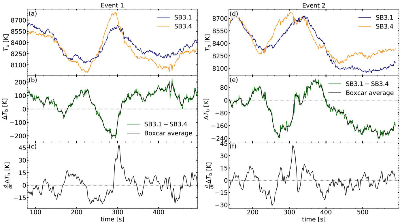
Fig. 12. Temporal evolution of the brightness temperatures at of the two selected brightening in the observational data. Left column: Event 1, Right column: Event 2. The locations of the events are indicated in the FOV of Fig. 11. (a,d) Brightness temperatures of SB3.1 and SB3.4. (b,e) Brightness temperature differences between the sub-bands \Delta T_{b|B3} . Green graph shows the original data and black curve a boxcar average over 10 s. (c,f) The time derivative of the (boxcar averaged) sub-band differences.
